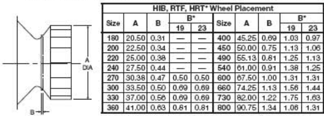
Figure 6. Wheel-Funnel Overlap
