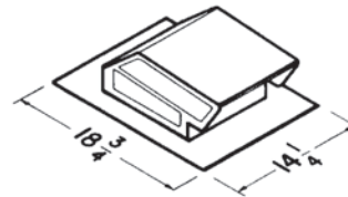
Model 634 Roof Cap • Black electrically - bonded epoxy finish • Built-in backdraft damper & birdscreen • For 3 1/4" x 10" or up to 8" round duct
