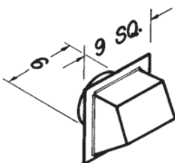
Model 641 Wall Cap • Aluminum natural finish • Built-in backdraft damper & birdscreen • For 6" round duct
