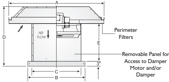
Model HRSB-F Filtered Belt Drive Model HRSD-F Filtered Direct Dive
