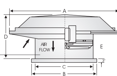
Model HRSB Supply Belt Drive Model HRSD Supply Direct Dive
