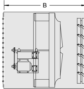
SIDE VIEW Shown with Motorside Wire Guard and Gravity Exhaust Damper
